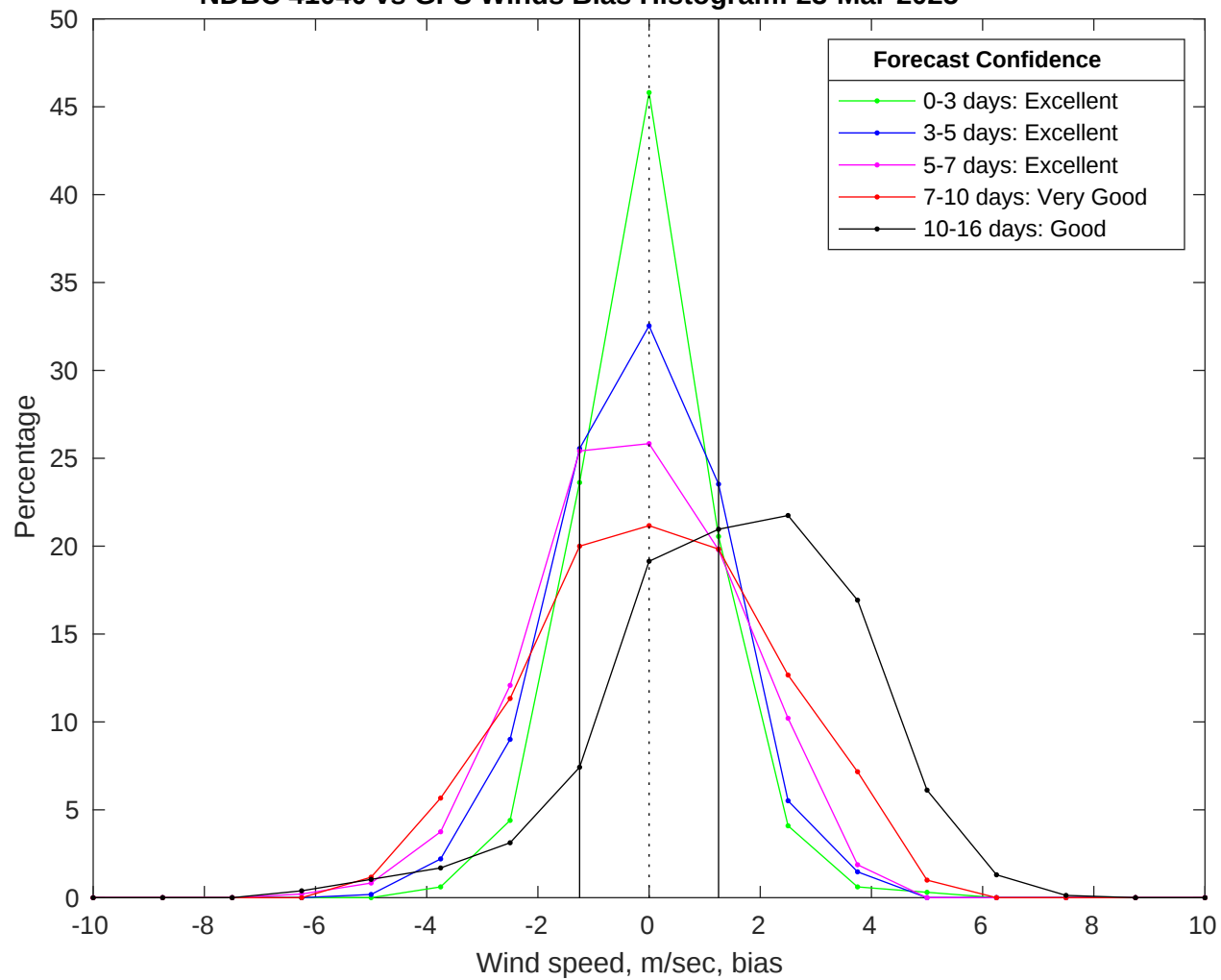
NDBC 41040 vs GFS Winds Bias Histogram: 23-Mar-2025
