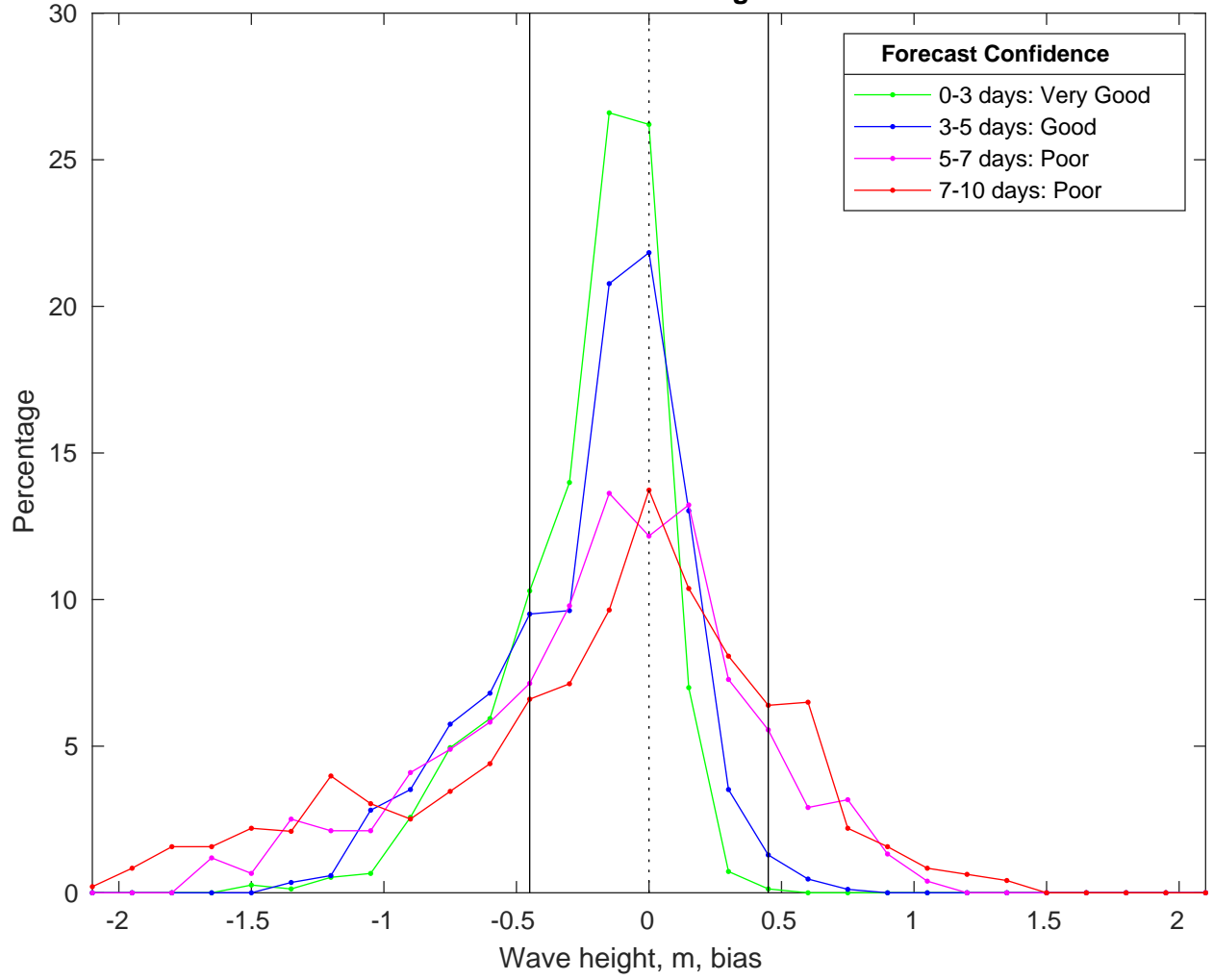
NDBC 42019 vs CMEMS Waves Bias Histogram: 23-Mar-2025
