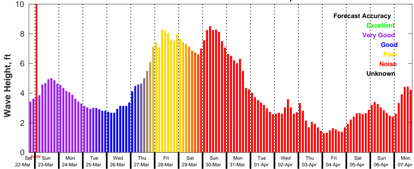
GFS Wave Forecast for NDBC 42019 from 22-Mar-2025 18:00:00 to 07-Apr-2025 18:00:00
