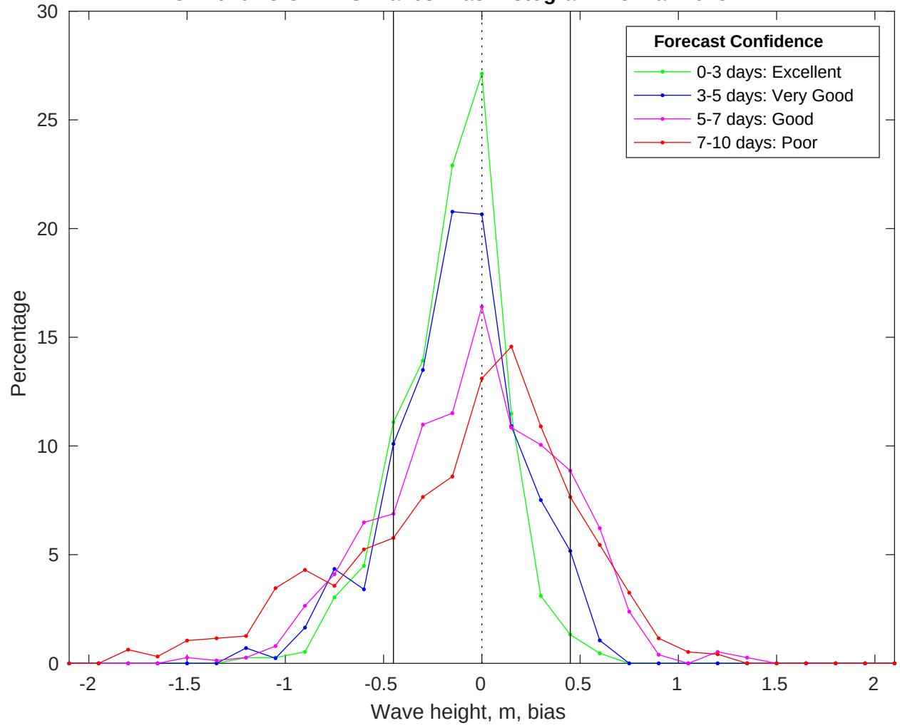
NDBC 42020 vs CMEMS Waves Bias Histogram: 23-Mar-2025
