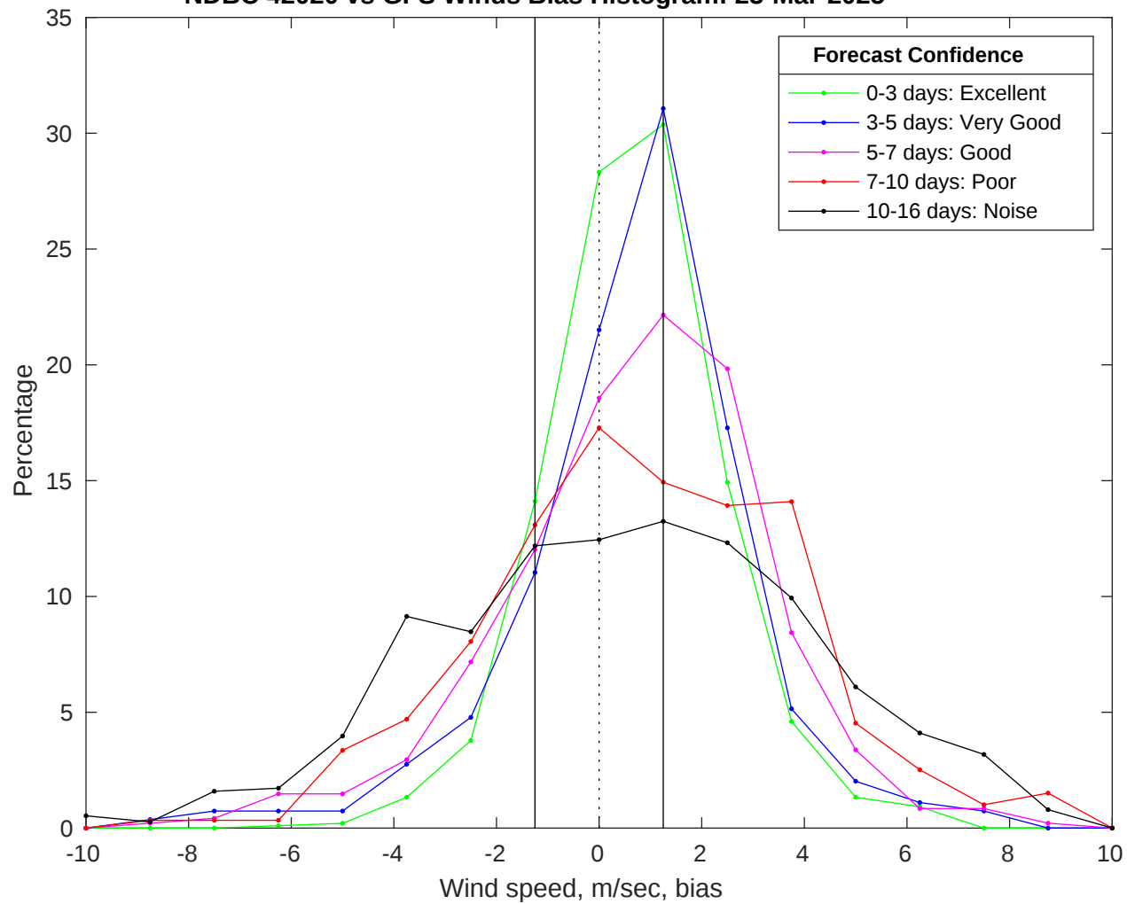
NDBC 42020 vs GFS Winds Bias Histogram: 23-Mar-2025
