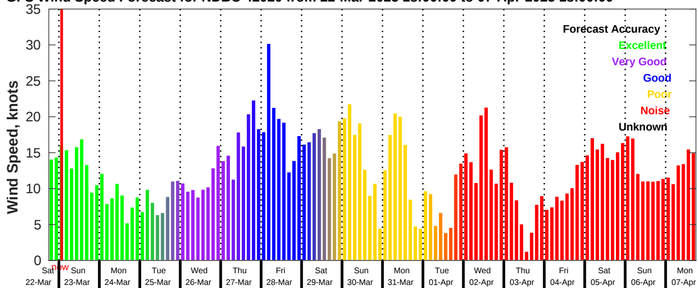
GFS Wind Speed Forecast for NDBC 42020 from 22-Mar-2025 18:00:00 to 07-Apr-2025 18:00:00
