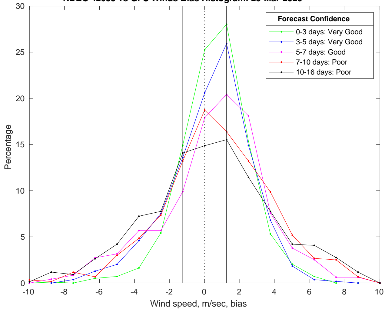
NDBC 42035 vs GFS Winds Bias Histogram: 23-Mar-2025
