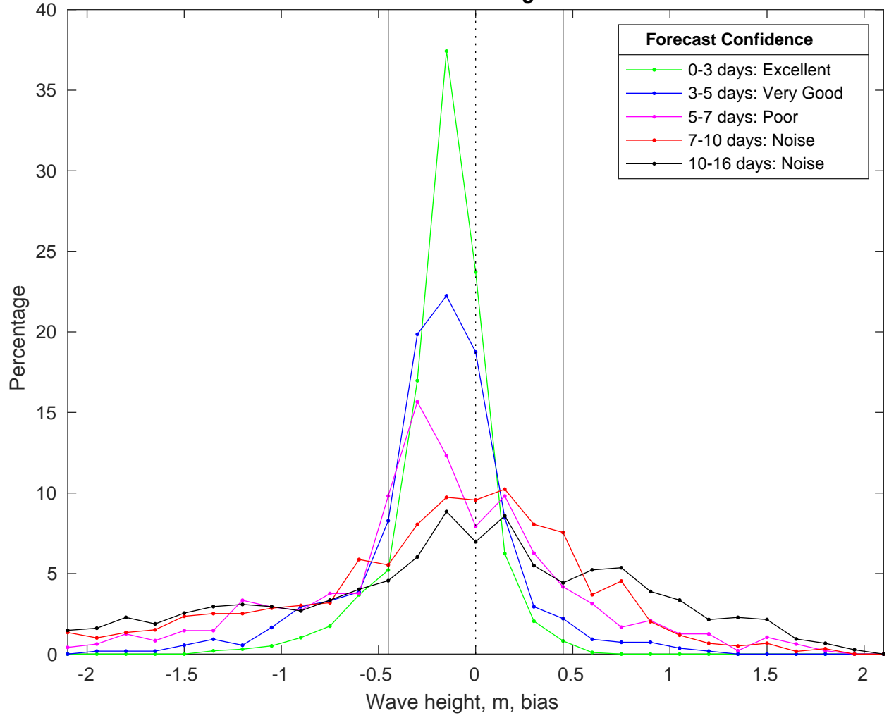
NDBC 42036 vs GFS Waves Bias Histogram: 23-Mar-2025
