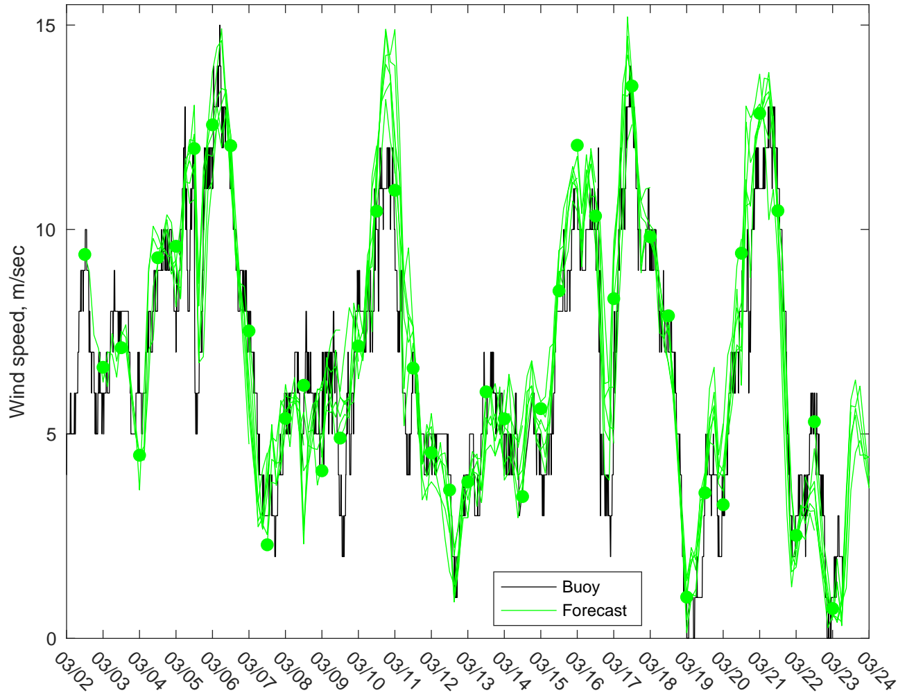
NDBC 42036 vs GFS Winds: 0 to 3 day forecast
