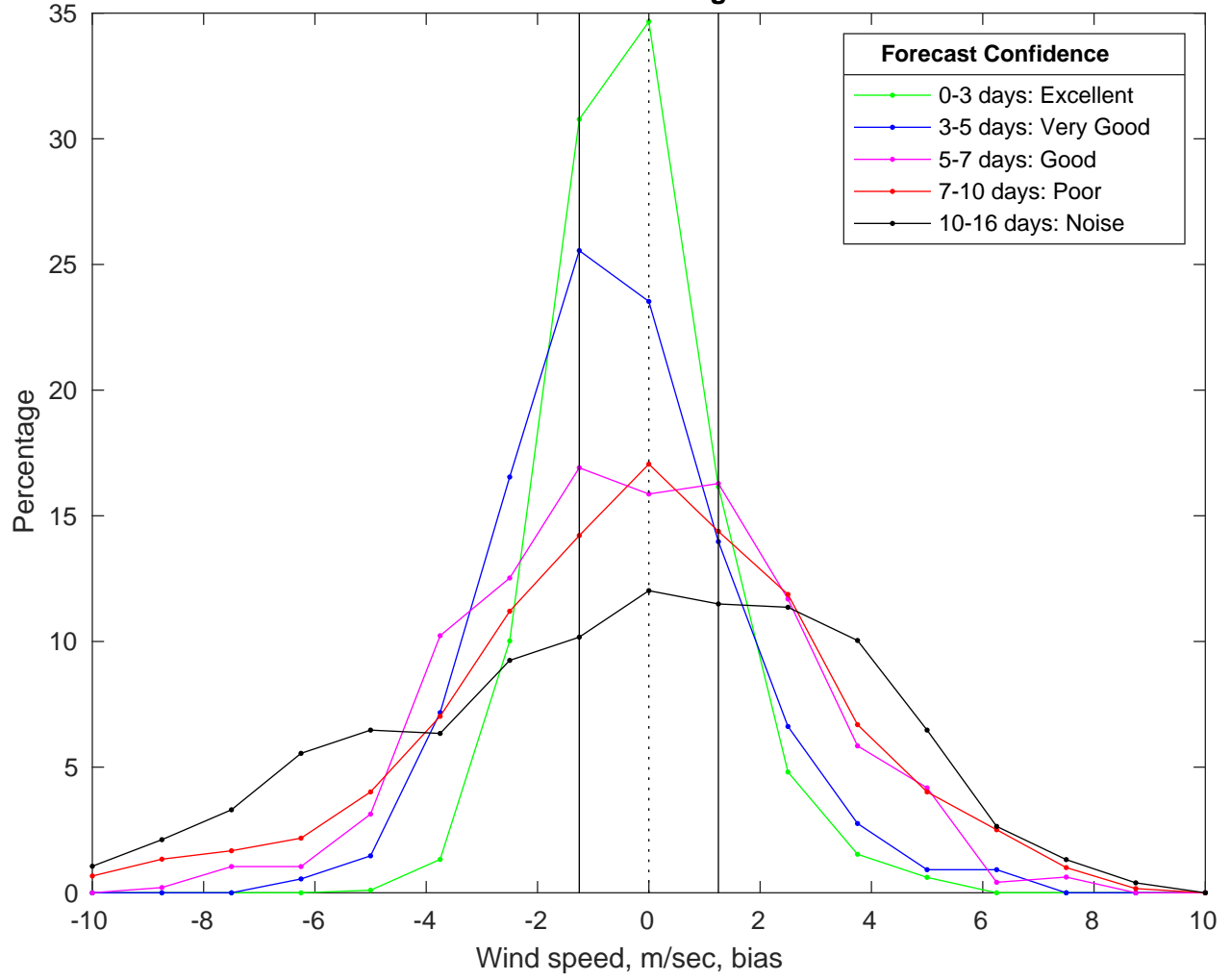
NDBC 42036 vs GFS Winds Bias Histogram: 23-Mar-2025
