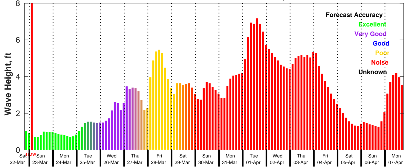
GFS Wave Forecast for NDBC 42036 from 22-Mar-2025 19:00:00 to 07-Apr-2025 19:00:00
