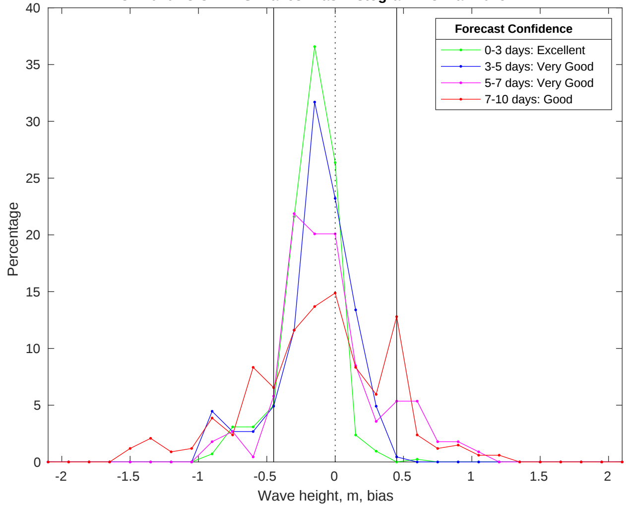
NDBC 42040 vs CMEMS Waves Bias Histogram: 23-Mar-2025
