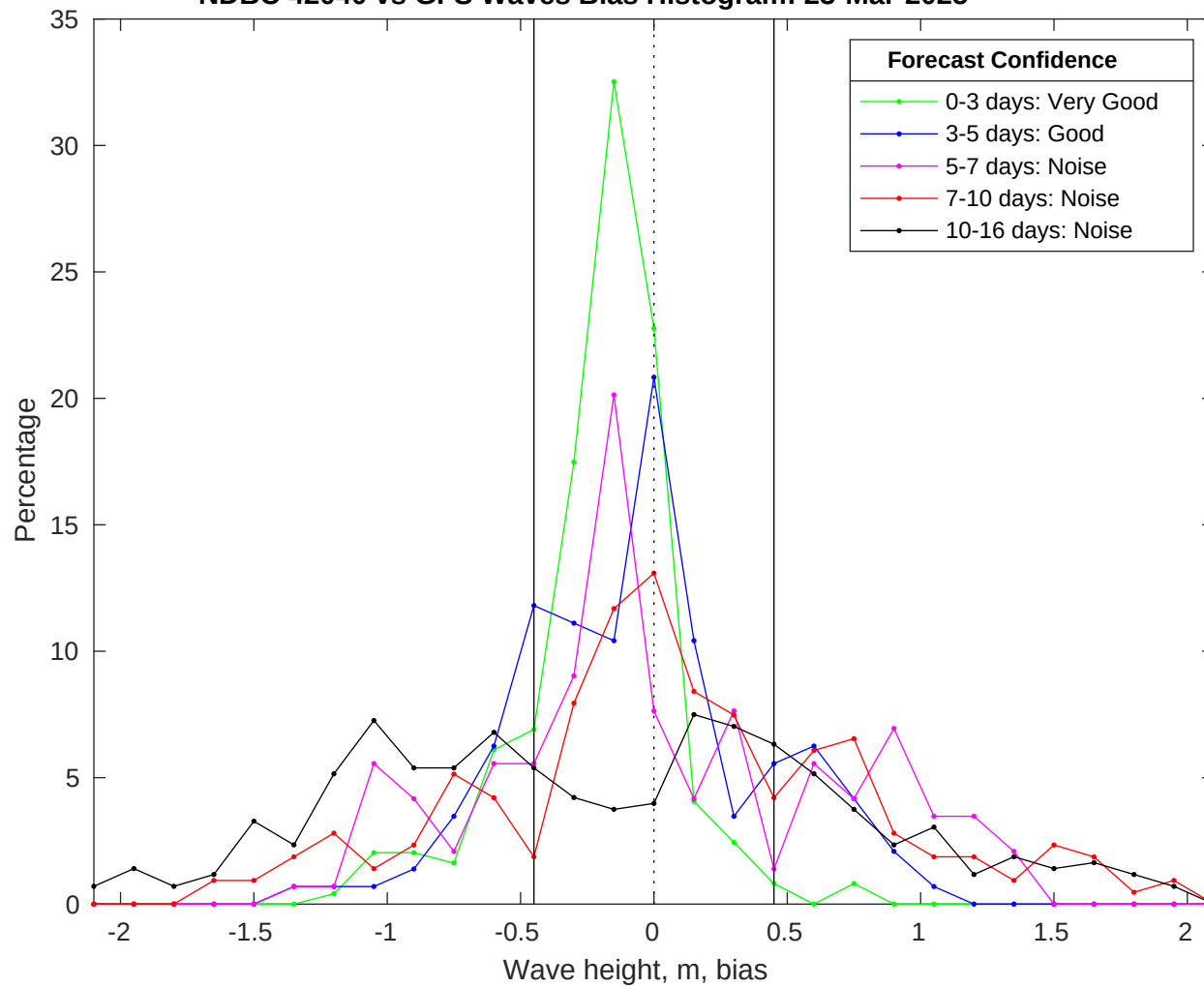
NDBC 42040 vs GFS Waves Bias Histogram: 23-Mar-2025
