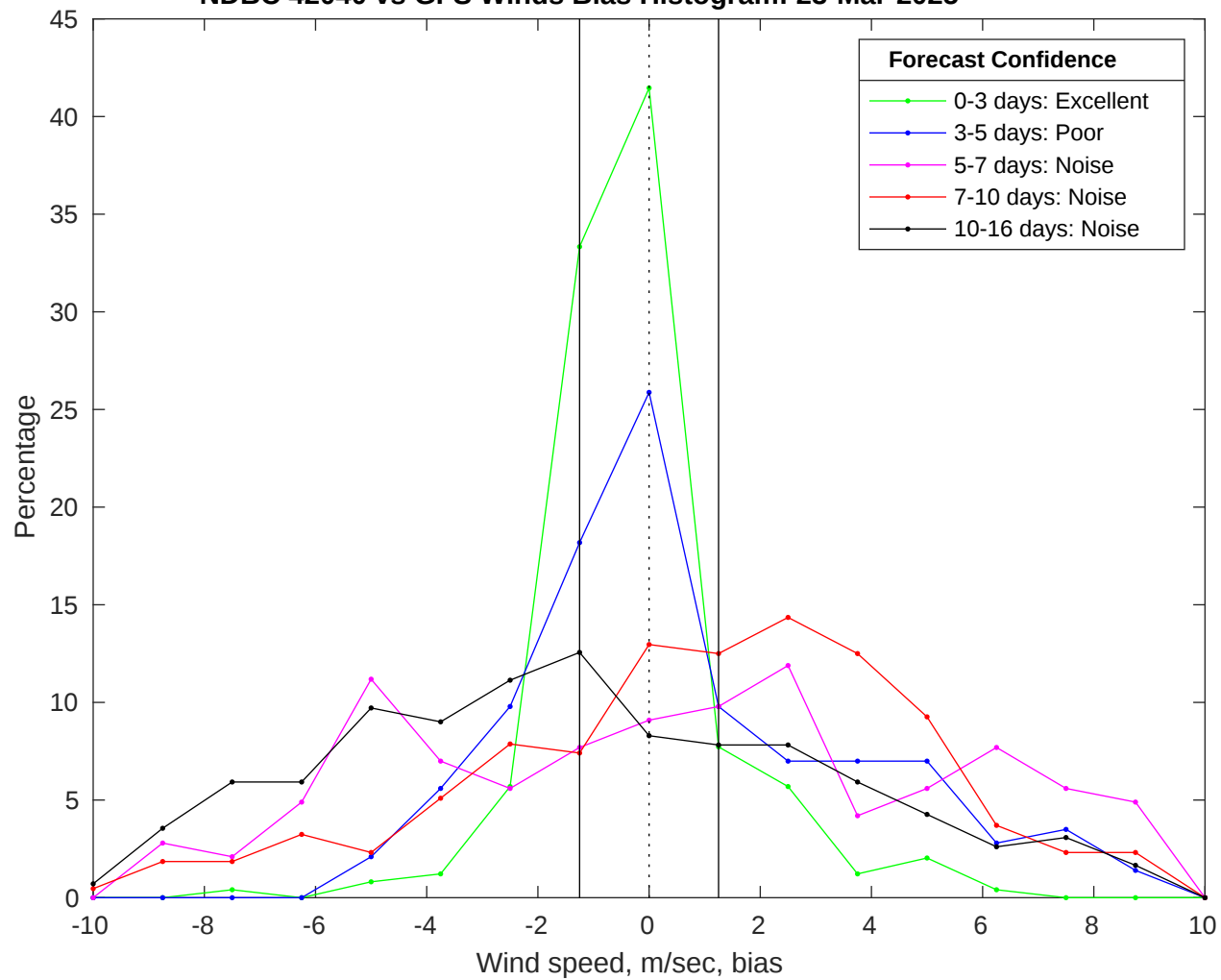
NDBC 42040 vs GFS Winds Bias Histogram: 23-Mar-2025
