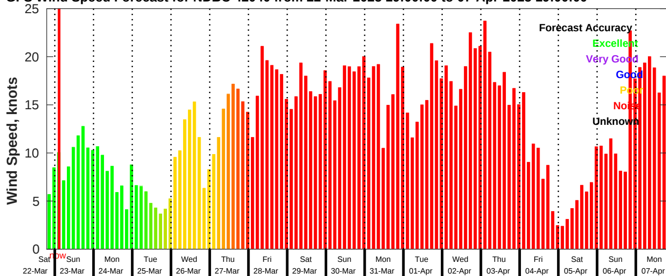
GFS Wind Speed Forecast for NDBC 42040 from 22-Mar-2025 19:00:00 to 07-Apr-2025 19:00:00
