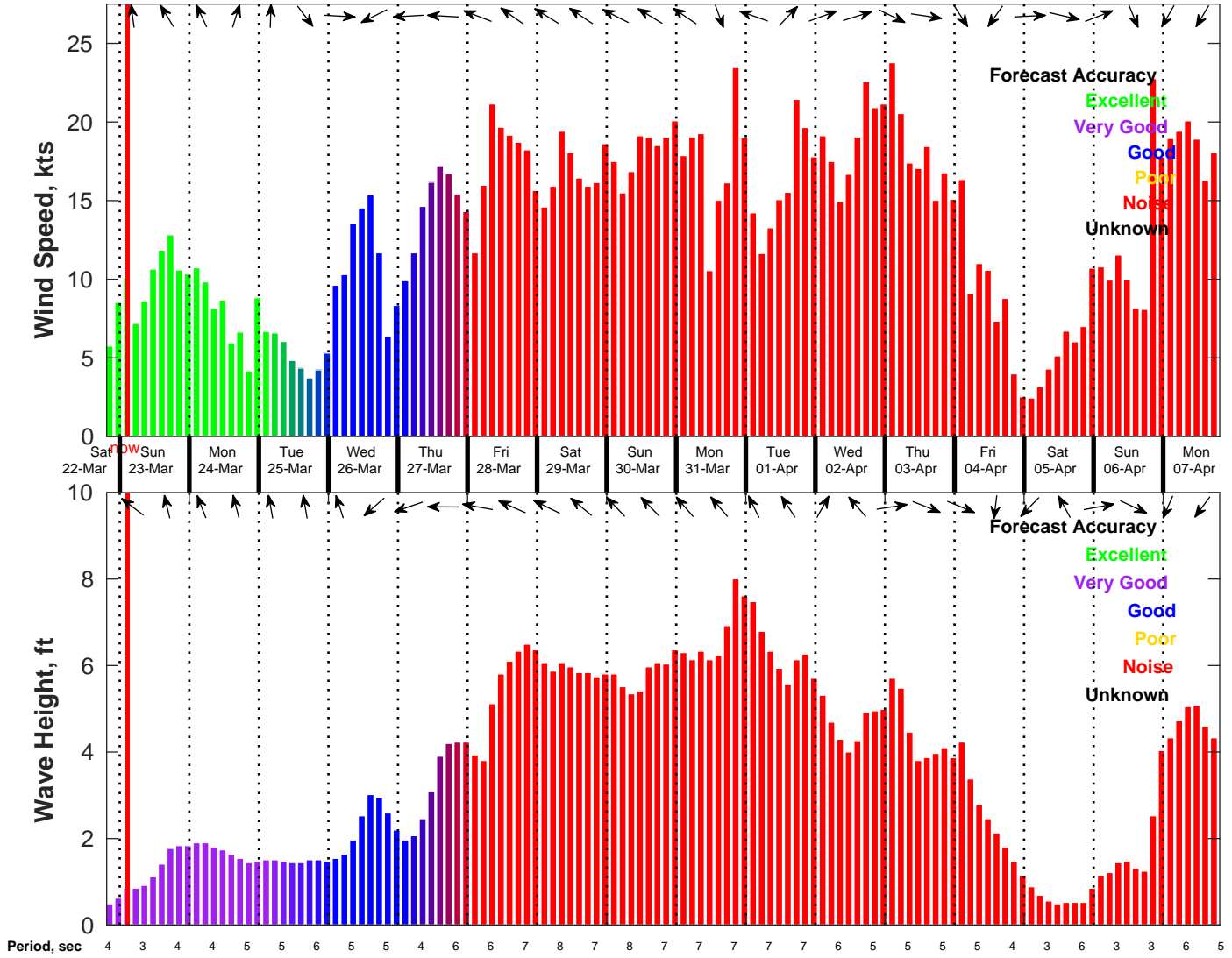
Wind & Wave Forecast for NDBC 42040 from 22-Mar-2025 19:00:00 to 07-Apr-2025 19:00:00
