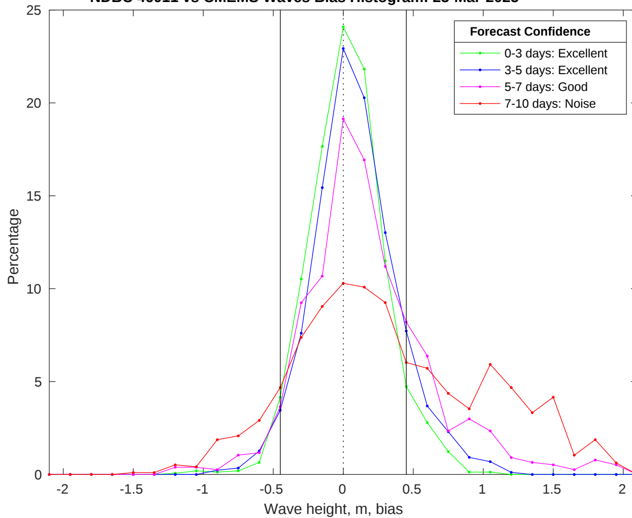
NDBC 46011 vs CMEMS Waves Bias Histogram: 23-Mar-2025
