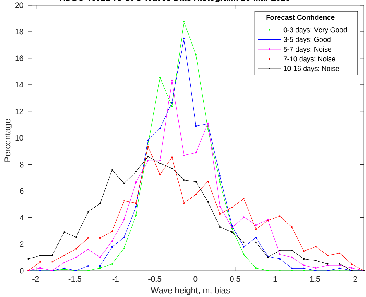
NDBC 46011 vs GFS Waves Bias Histogram: 23-Mar-2025
