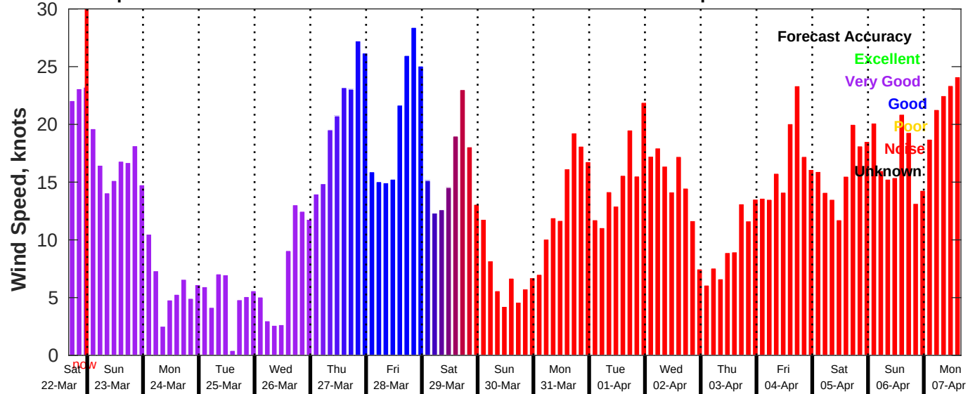
GFS Wind Speed Forecast for NDBC 46011 from 22-Mar-2025 16:00:00 to 07-Apr-2025 16:00:00
