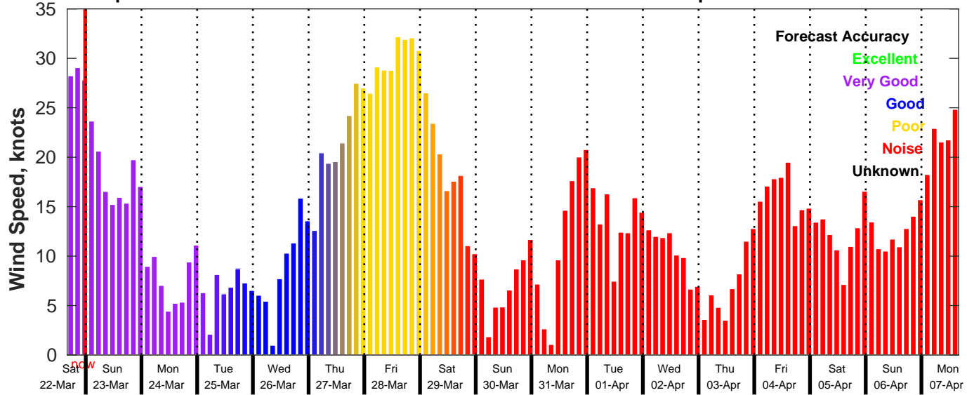
GFS Wind Speed Forecast for NDBC 46028 from 22-Mar-2025 16:00:00 to 07-Apr-2025 16:00:00
