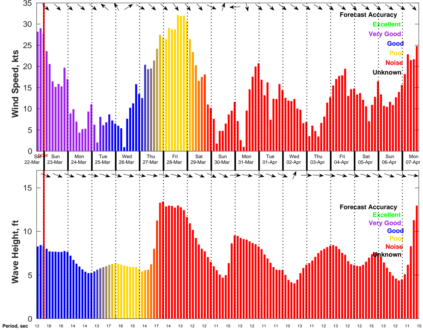
Wind & Wave Forecast for NDBC 46028 from 22-Mar-2025 16:00:00 to 07-Apr-2025 16:00:00
