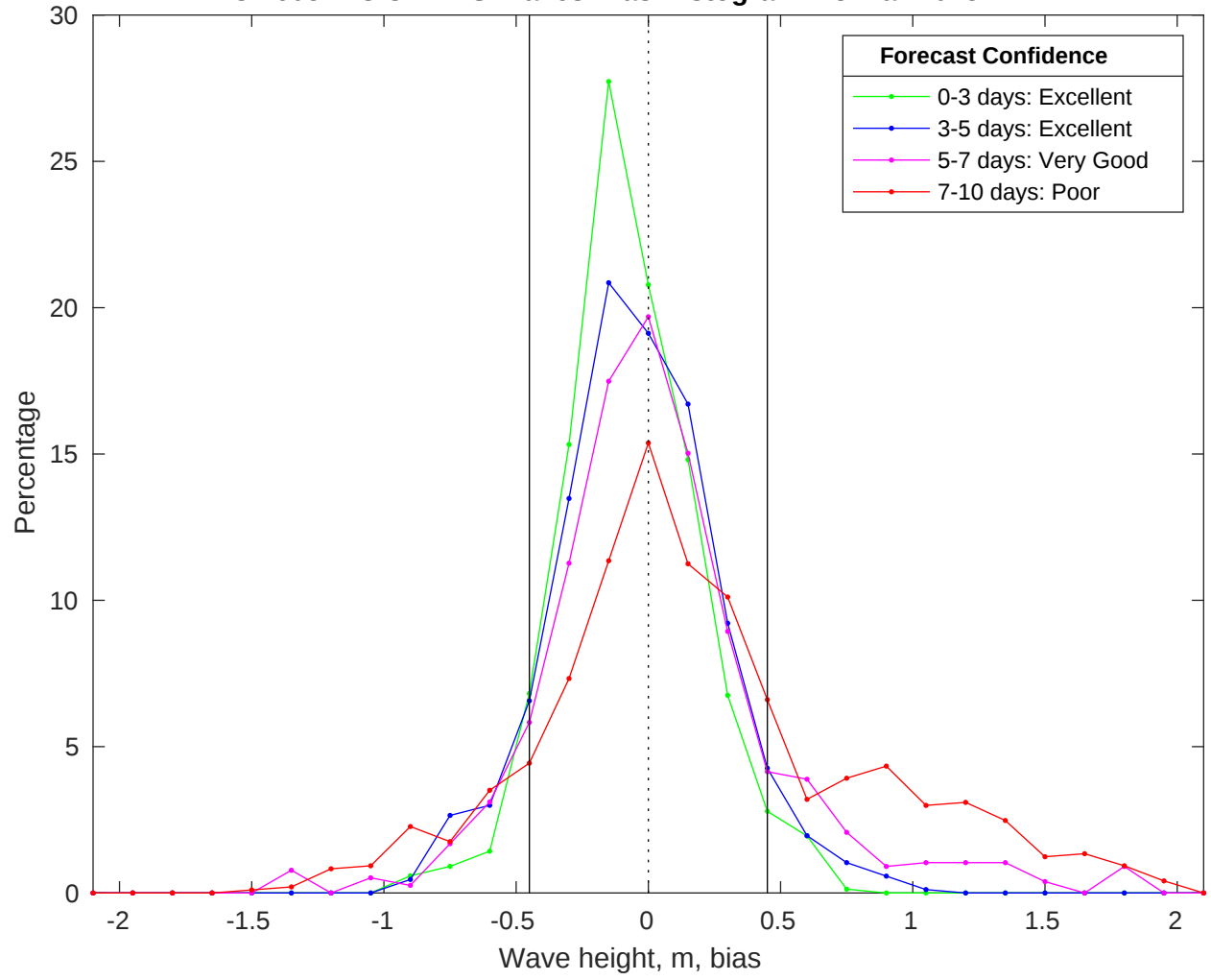
NDBC 46054 vs CMEMS Waves Bias Histogram: 23-Mar-2025
