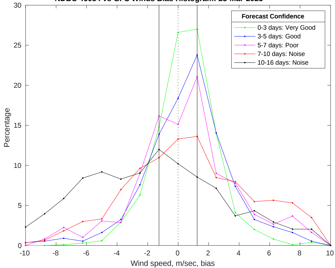
NDBC 46054 vs GFS Winds Bias Histogram: 23-Mar-2025
