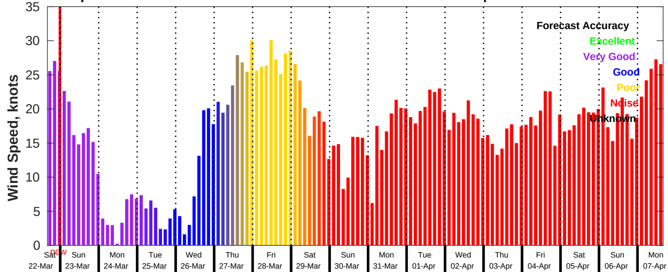
GFS Wind Speed Forecast for NDBC 46054 from 22-Mar-2025 16:00:00 to 07-Apr-2025 16:00:00
