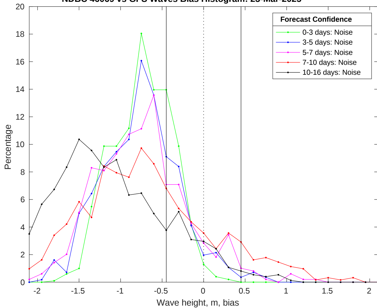
NDBC 46069 vs GFS Waves Bias Histogram: 23-Mar-2025
