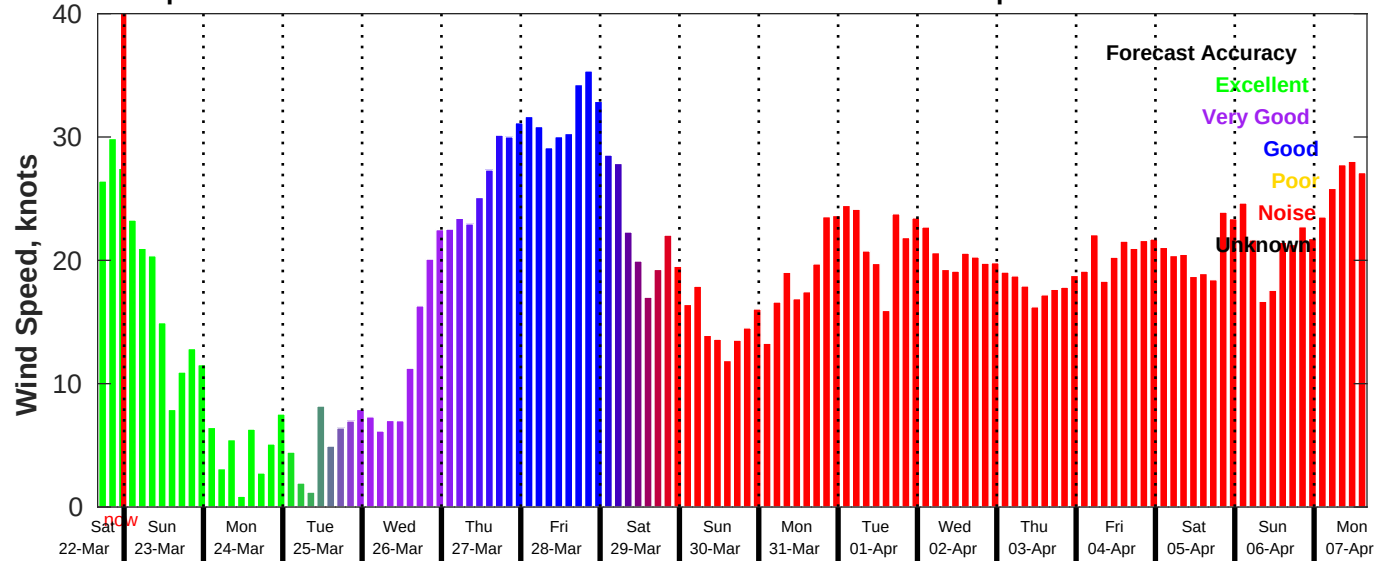
GFS Wind Speed Forecast for NDBC 46069 from 22-Mar-2025 16:00:00 to 07-Apr-2025 16:00:00
