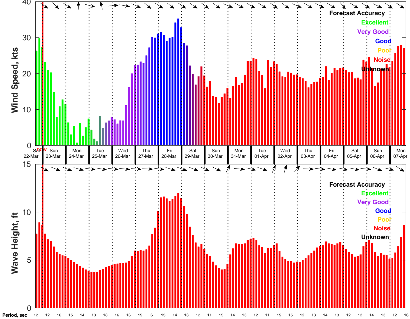
Wind & Wave Forecast for NDBC 46069 from 22-Mar-2025 16:00:00 to 07-Apr-2025 16:00:00
