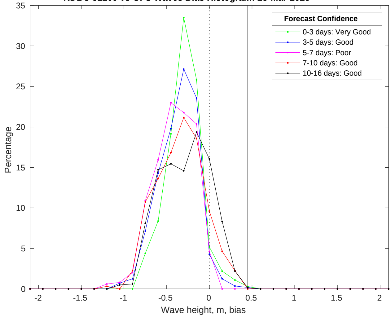
NDBC 51209 vs GFS Waves Bias Histogram: 23-Mar-2025
