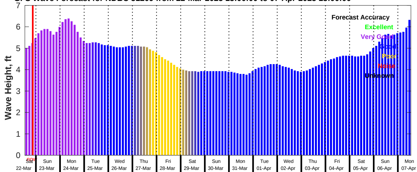
GFS Wave Forecast for NDBC 51209 from 22-Mar-2025 13:00:00 to 07-Apr-2025 13:00:00
