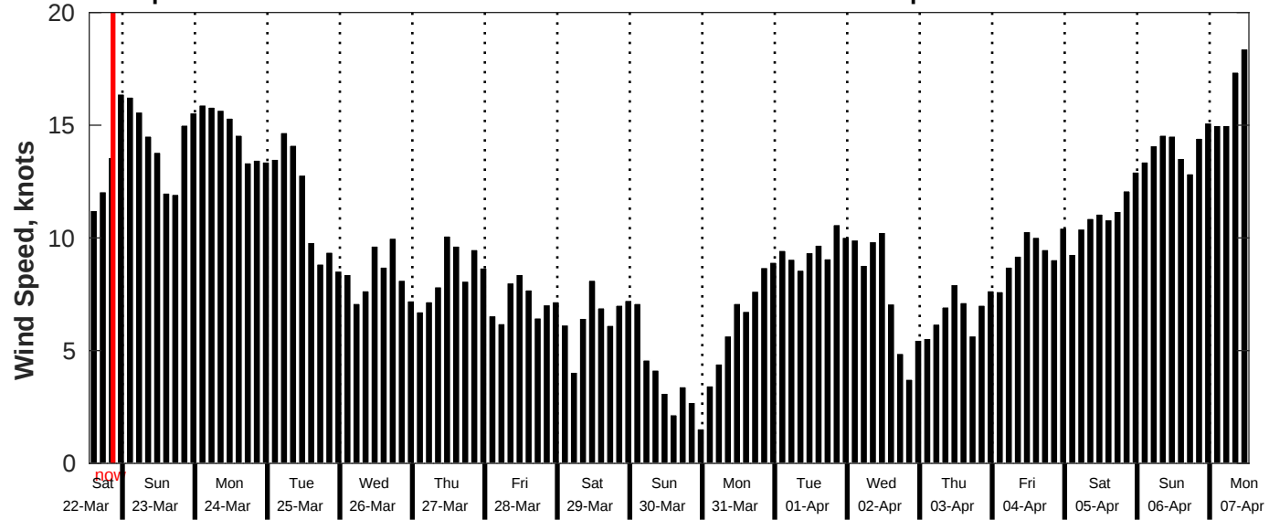
GFS Wind Speed Forecast for NDBC 51209 from 22-Mar-2025 13:00:00 to 07-Apr-2025 13:00:00
