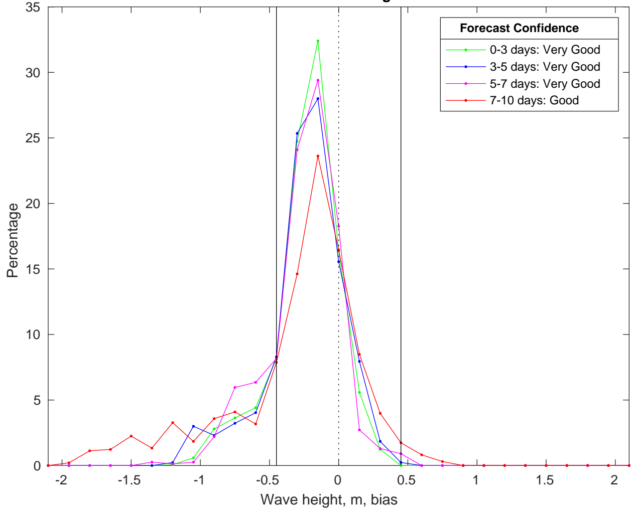
NDBC 52211 vs CMEMS Waves Bias Histogram: 23-Mar-2025
