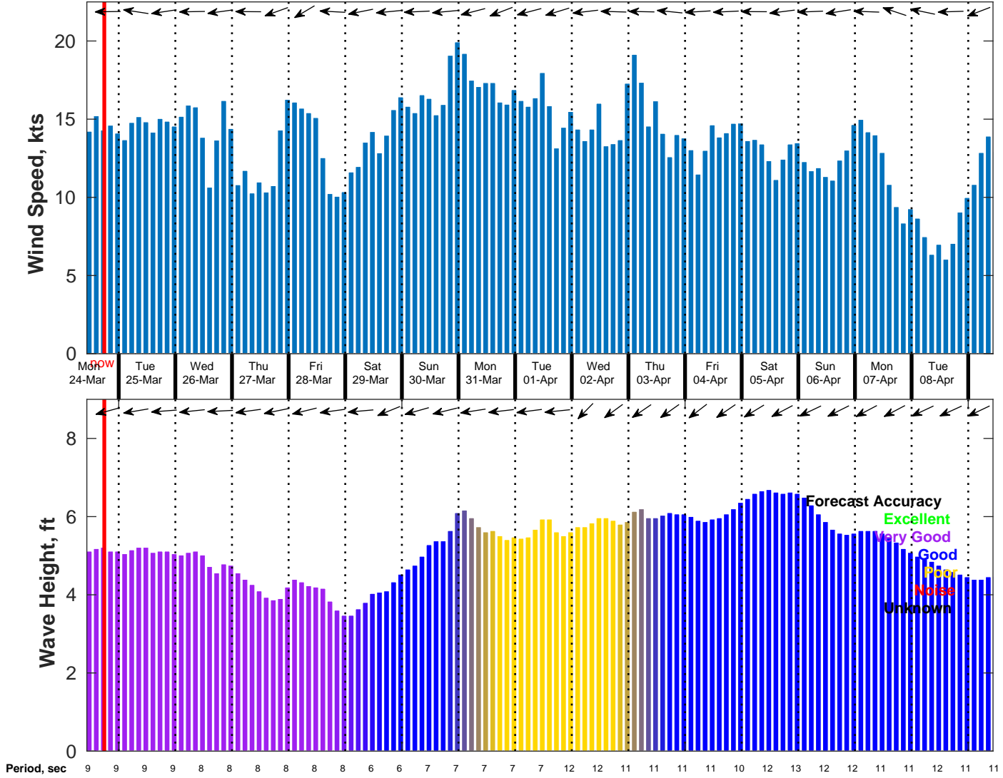
Wind & Wave Forecast for NDBC 52211 from 23-Mar-2025 10:00:00 to 08-Apr-2025 10:00:00
