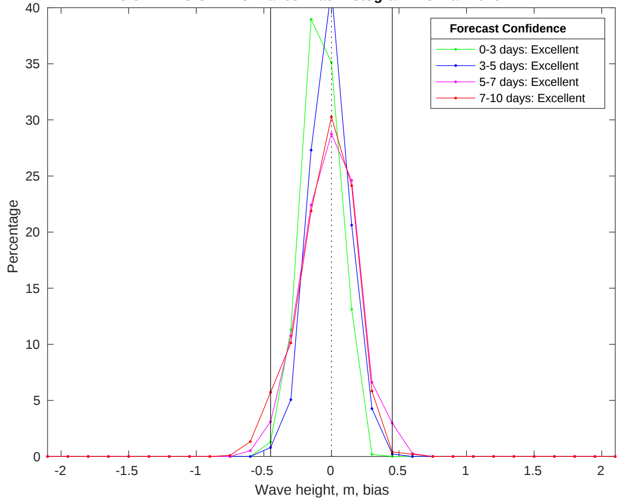
NDBC 52212 vs CMEMS Waves Bias Histogram: 23-Mar-2025
