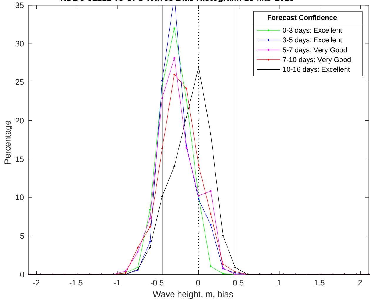
NDBC 52212 vs GFS Waves Bias Histogram: 23-Mar-2025
