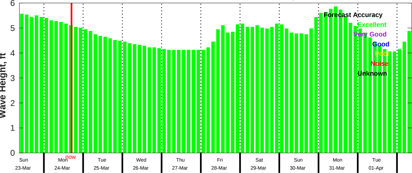
CMEMS Wave Forecast for NDBC 52212 from 22-Mar-2025 09:00:00 to 01-Apr-2025 09:00:00
