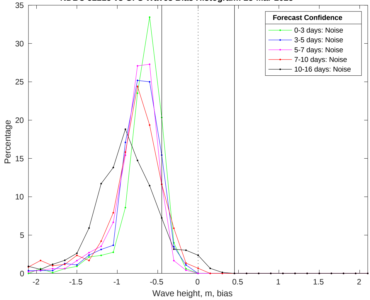
NDBC 52213 vs GFS Waves Bias Histogram: 23-Mar-2025
