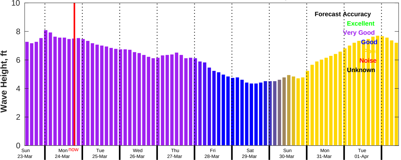
CMEMS Wave Forecast for NDBC 52213 from 22-Mar-2025 11:00:00 to 01-Apr-2025 11:00:00
