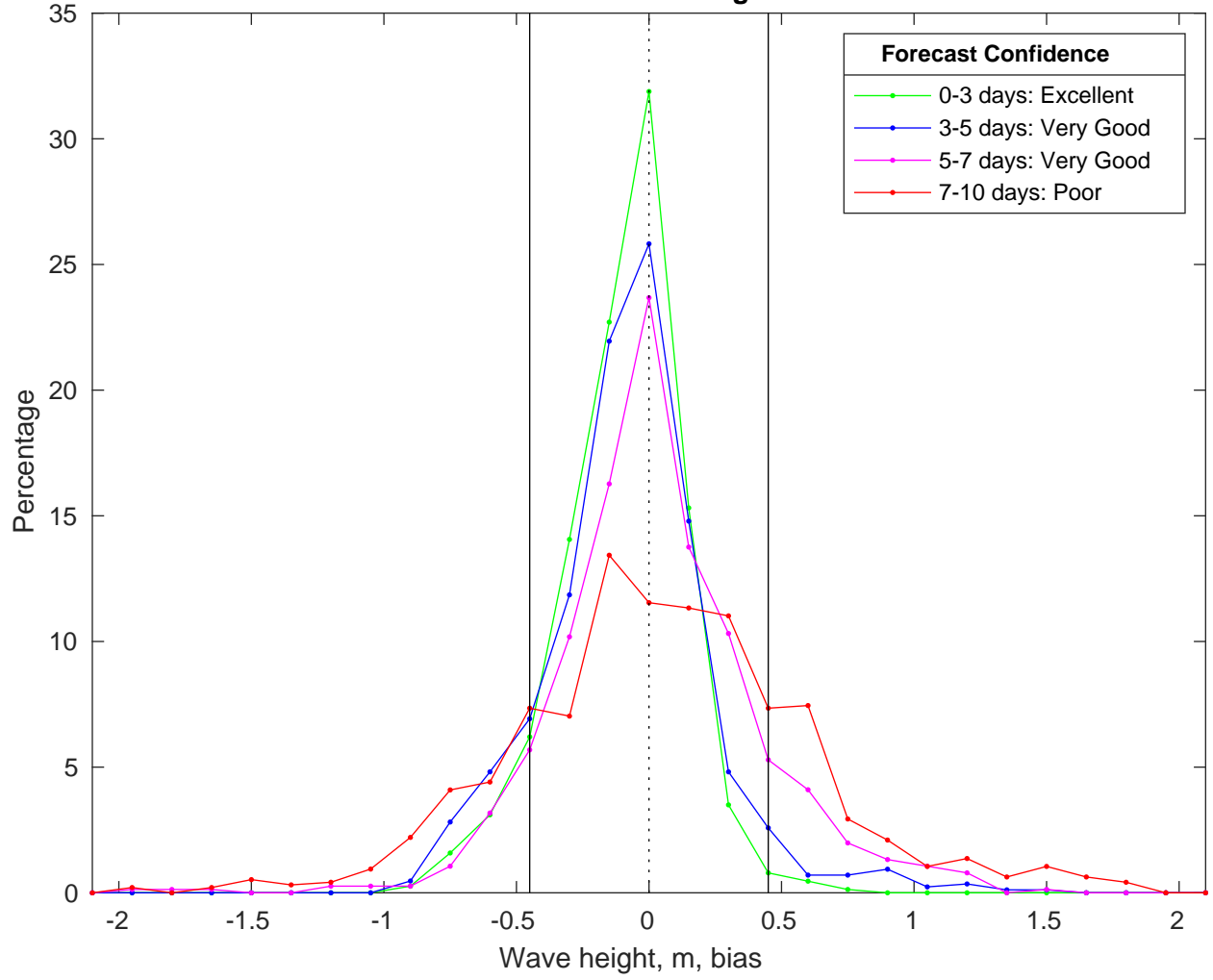
NDBC 41004 vs CMEMS Waves Bias Histogram: 24-Mar-2025
