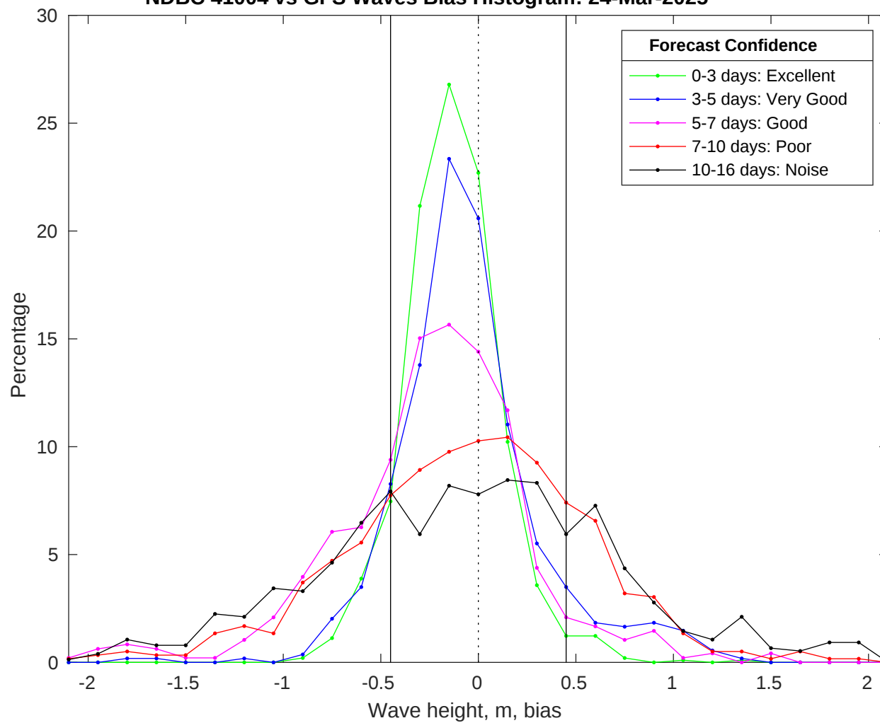
NDBC 41004 vs GFS Waves Bias Histogram: 24-Mar-2025
