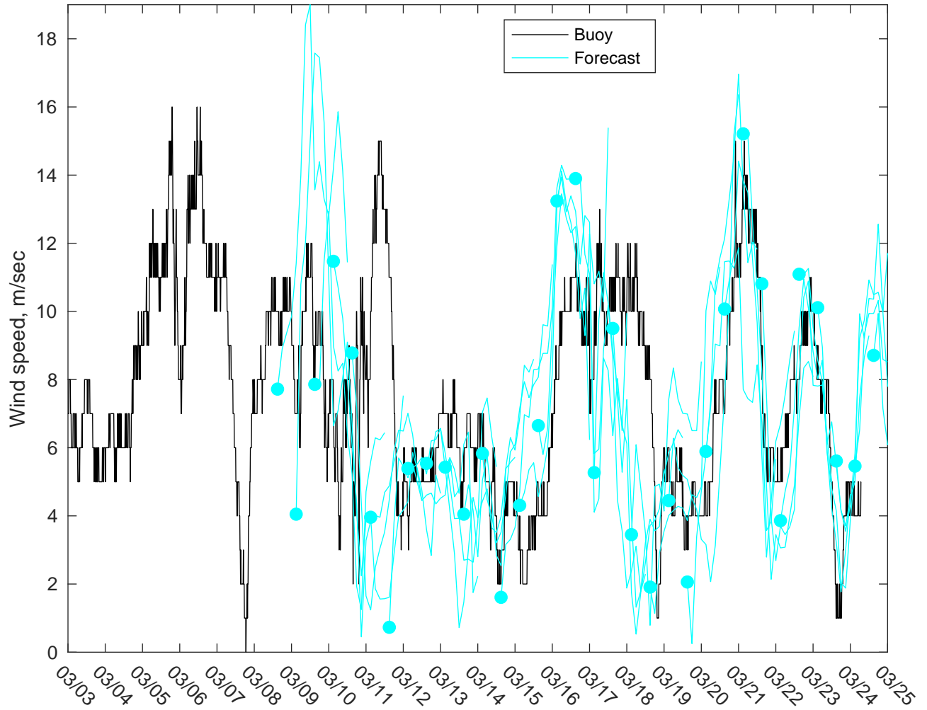
NDBC 41004 vs GFS Winds: 5 to 7 day forecast
