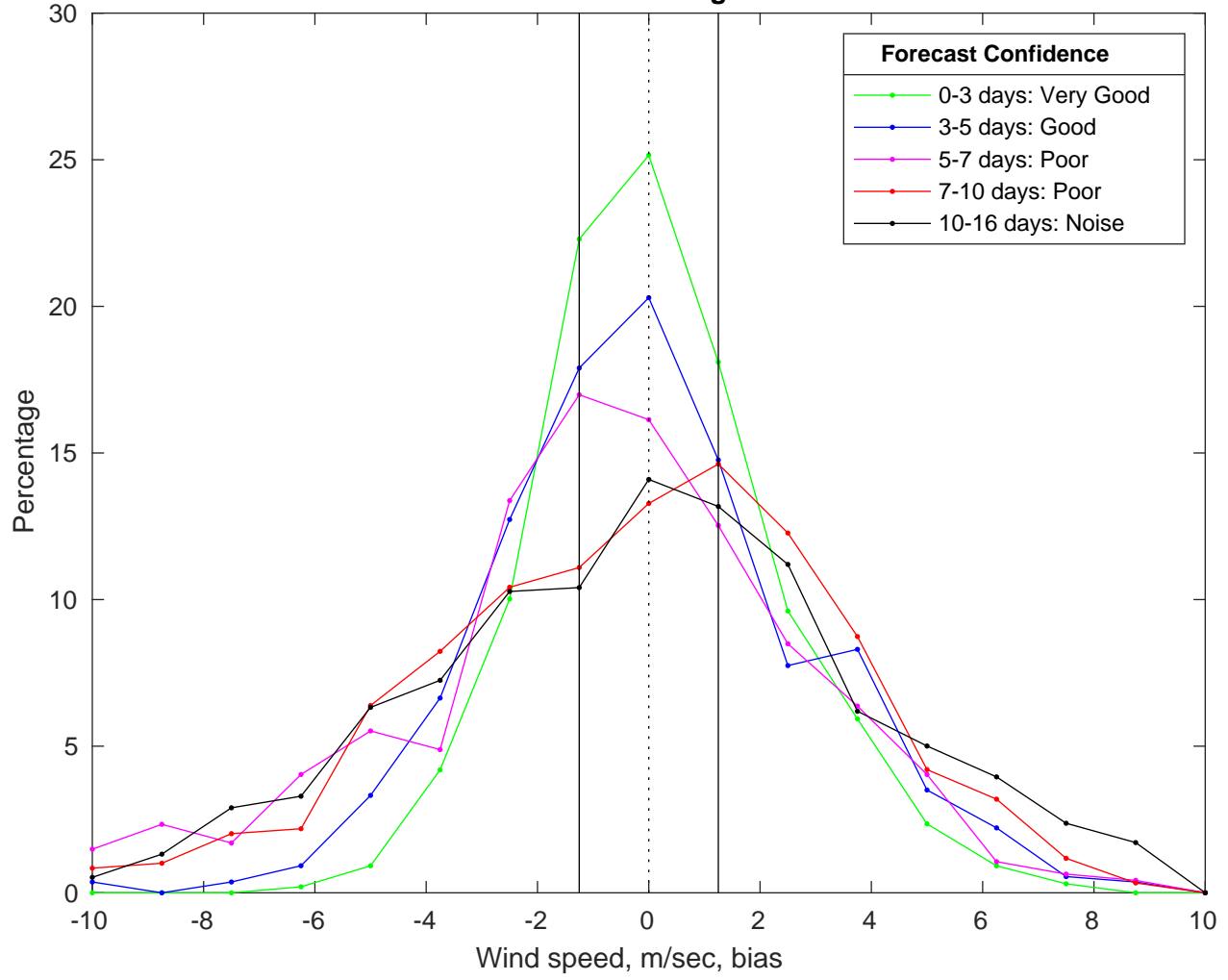
NDBC 41004 vs GFS Winds Bias Histogram: 24-Mar-2025
