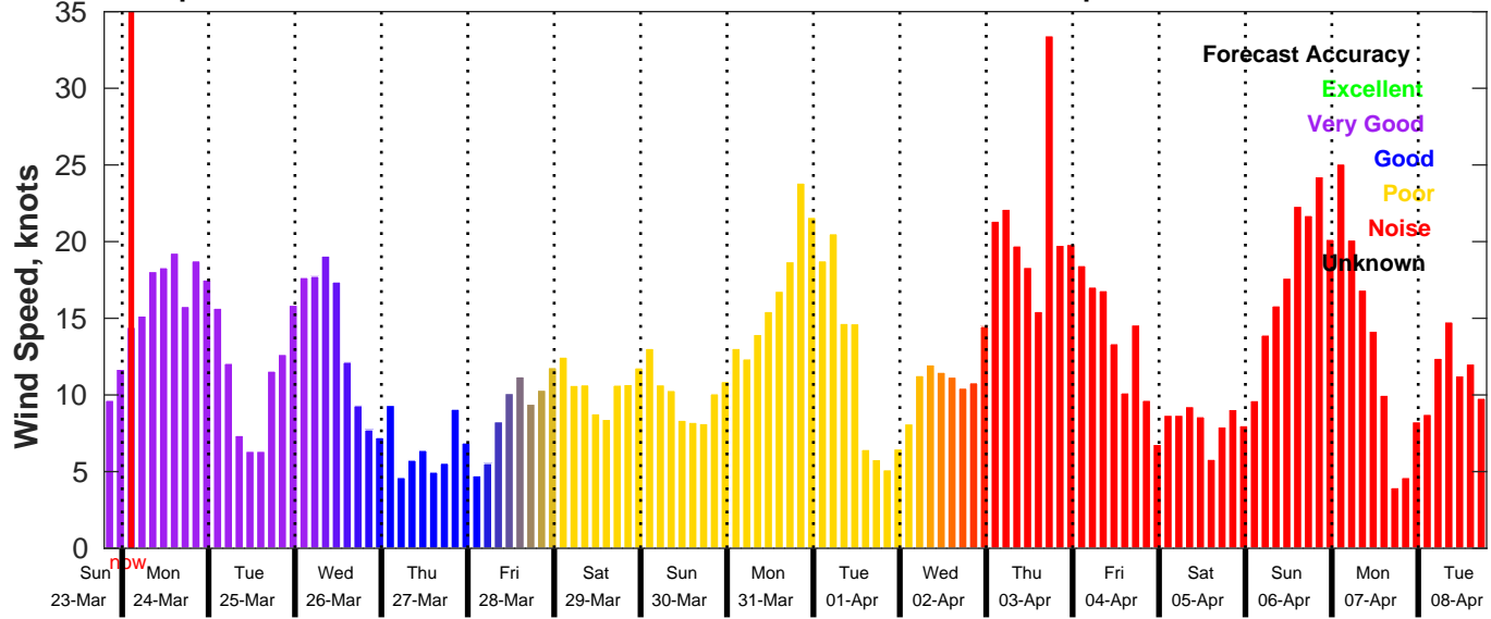
GFS Wind Speed Forecast for NDBC 41004 from 23-Mar-2025 19:00:00 to 08-Apr-2025 19:00:00
