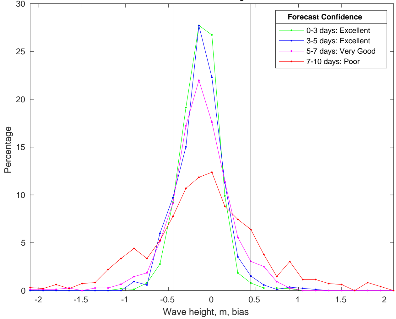
NDBC 41013 vs CMEMS Waves Bias Histogram: 24-Mar-2025
