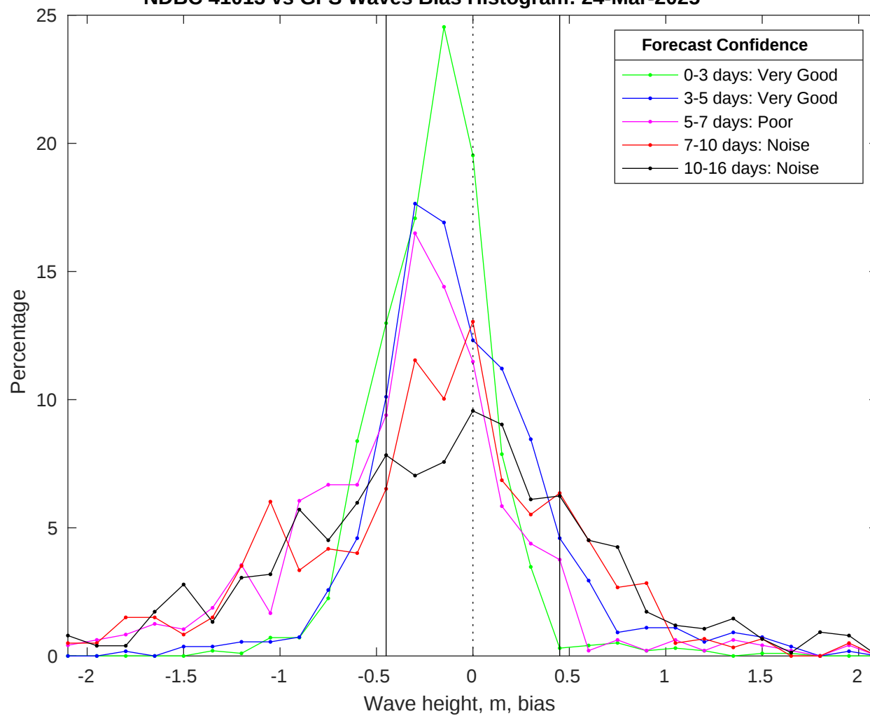
NDBC 41013 vs GFS Waves Bias Histogram: 24-Mar-2025
