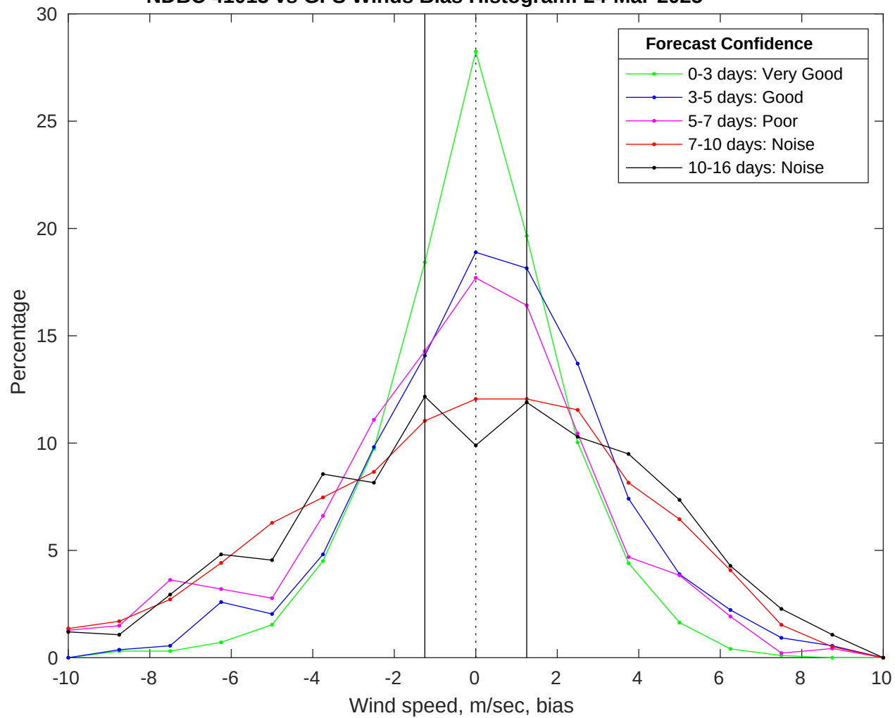
NDBC 41013 vs GFS Winds Bias Histogram: 24-Mar-2025
