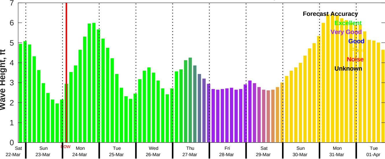
CMEMS Wave Forecast for NDBC 41013 from 22-Mar-2025 19:00:00 to 01-Apr-2025 19:00:00
