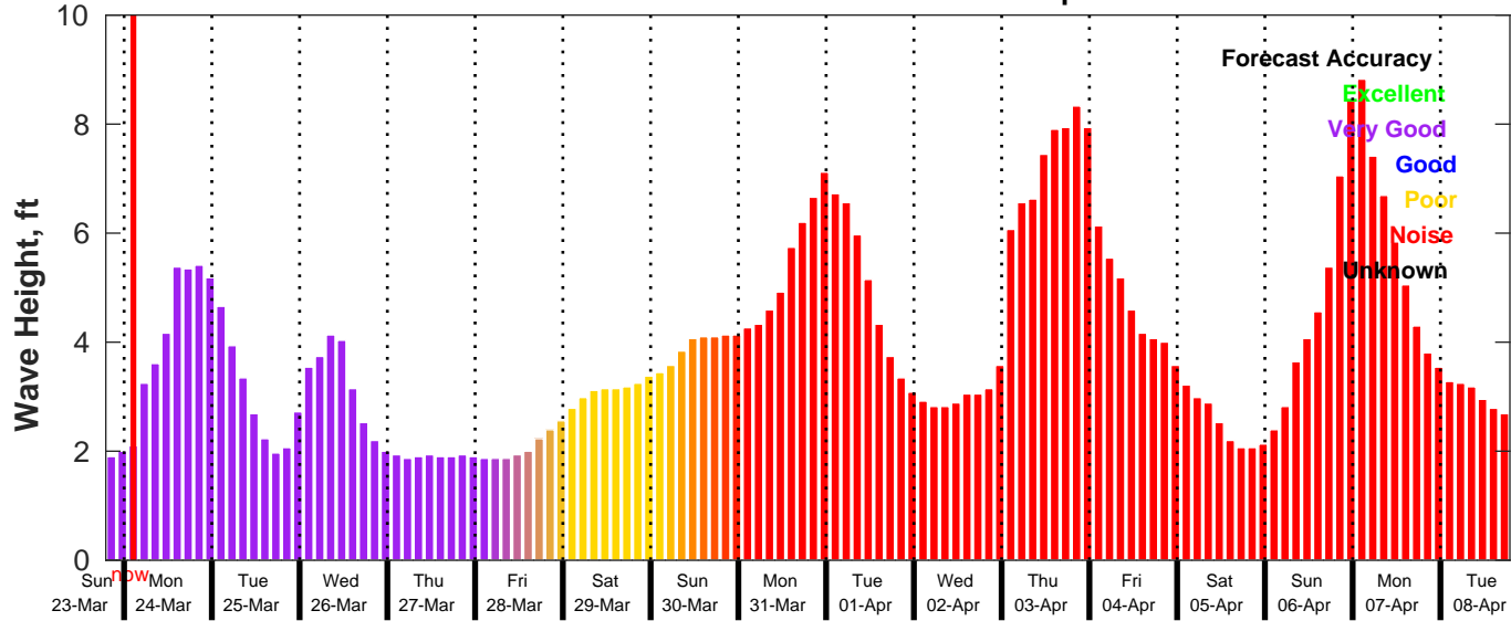
GFS Wave Forecast for NDBC 41013 from 23-Mar-2025 19:00:00 to 08-Apr-2025 19:00:00
