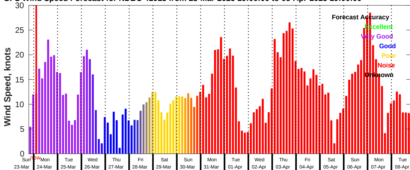
GFS Wind Speed Forecast for NDBC 41013 from 23-Mar-2025 19:00:00 to 08-Apr-2025 19:00:00
