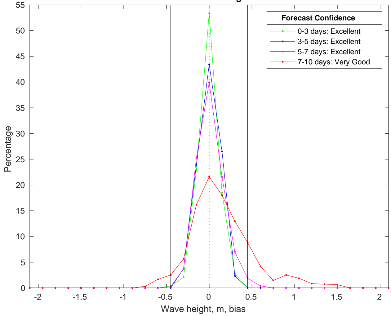
NDBC 41040 vs CMEMS Waves Bias Histogram: 24-Mar-2025
