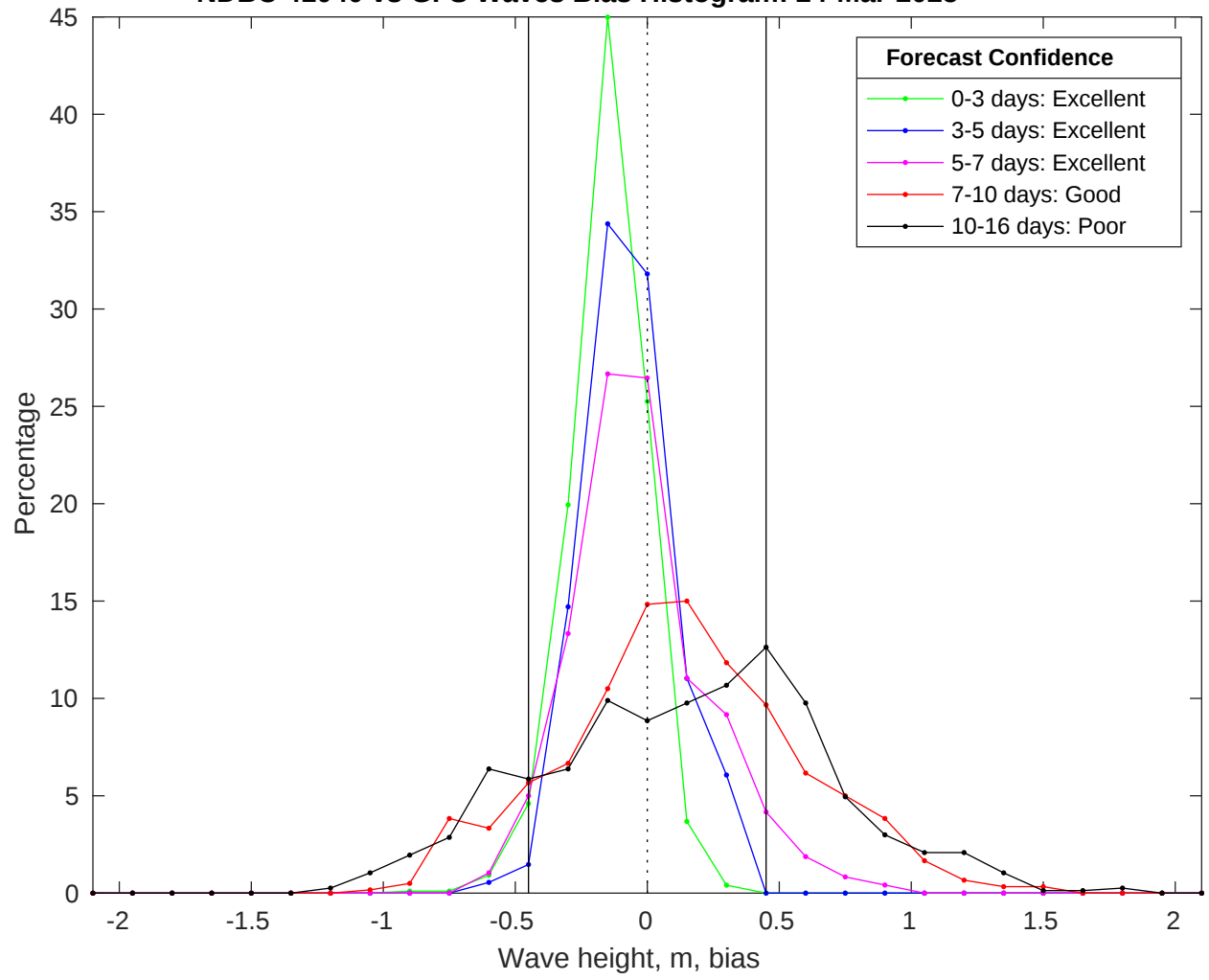
NDBC 41040 vs GFS Waves Bias Histogram: 24-Mar-2025
